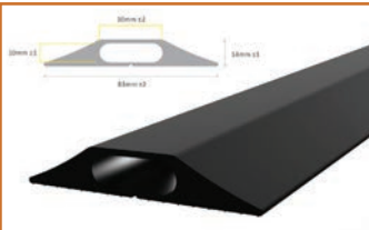
CablePRO GP - Black CP010013 & CP010006 Channel Size: 30mm W x 10mm H
